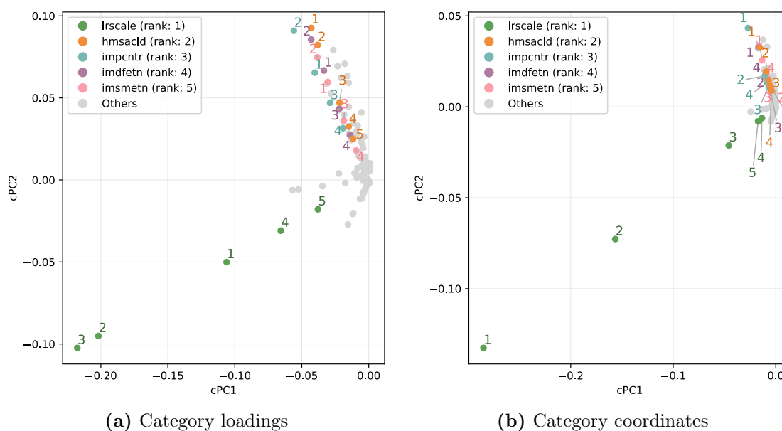
Fig. 25: Category loadings and coordinates of the top-5 variables along cPC2 (cMCA Con vs Lab, ESS 2018)
