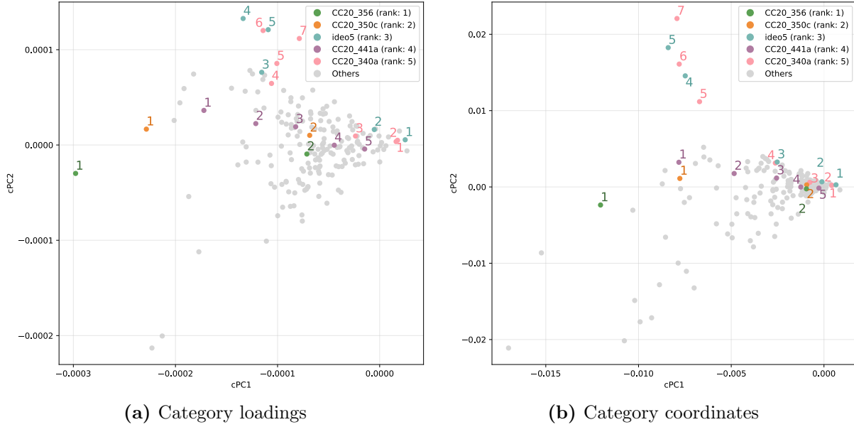
Fig. 18: Category loadings and coordinates of the top-5 variables along cPC1 (cMCA Dem vs Rep, CES 2020)
