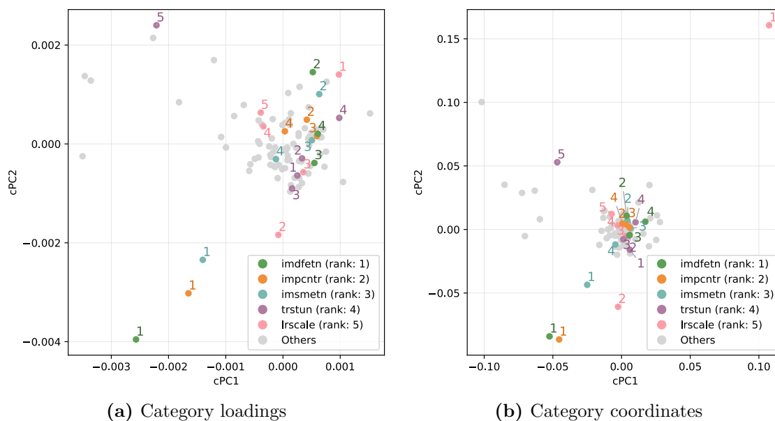
Fig. 29: Category loadings and coordinates of the top-5 variables along cPC2 (cMCA Con vs UKIP, ESS 2018)
