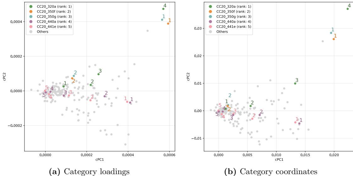
Fig. 20: Category loadings and coordinates of the top-5 variables along cPC1 (cMCA Rep vs Dem, CES 2020)
