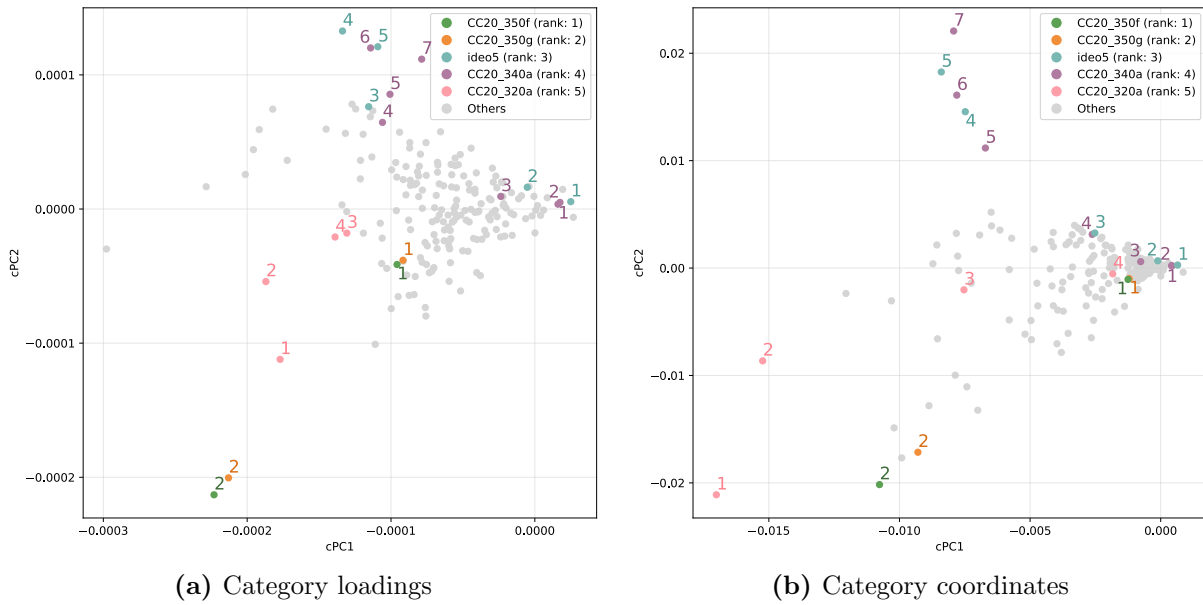
Fig. 19: Category loadings and coordinates of the top-5 variables along cPC2 (cMCA Dem vs Rep, CES 2020)
