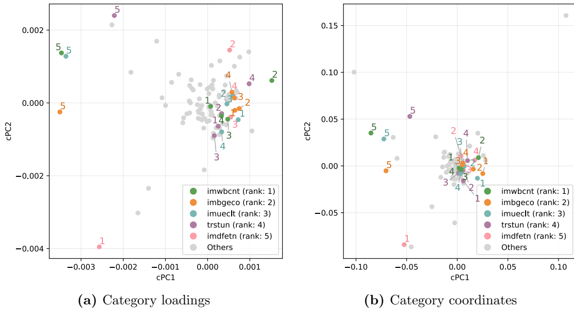
Fig. 28: Category loadings and coordinates of the top-5 variables along cPC1 (cMCA Con vs UKIP, ESS 2018)
