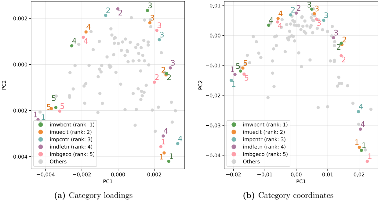
Fig. 17: Category loadings and coordinates of the top-5 variables in Table 11 (MCA, ESS 2018)
