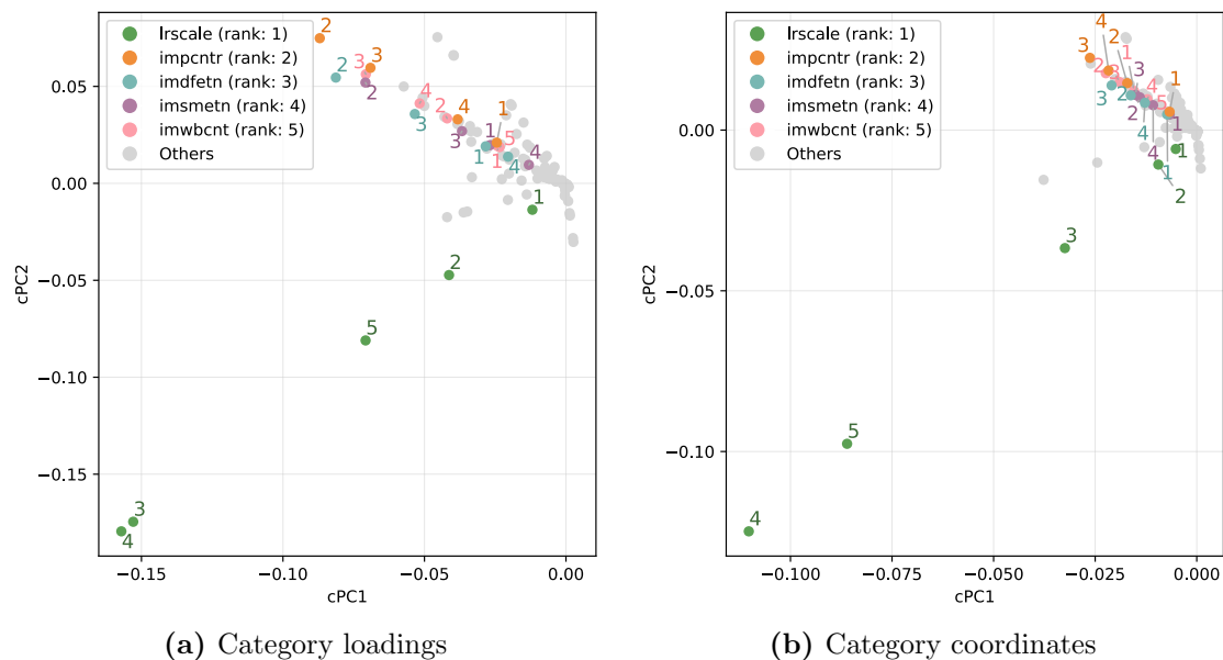
Fig. 22: Category loadings and coordinates of the top-5 variables along cPC1 (cMCA Lab vs Con, ESS 2018)
