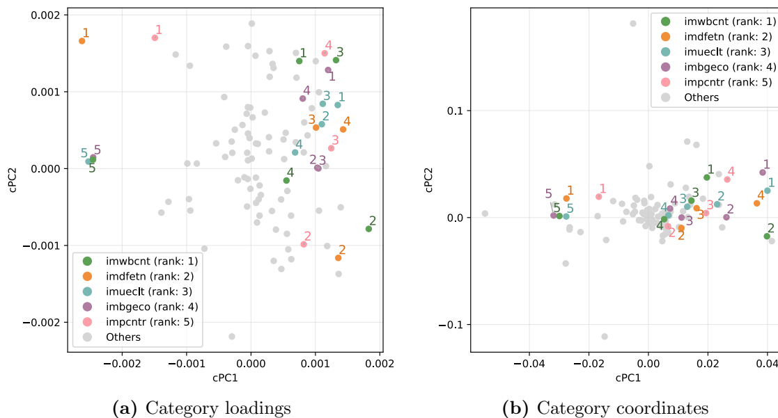
Fig. 26: Category loadings and coordinates of the top-5 variables along cPC1 (cMCA Lab vs UKIP, ESS 2018)
