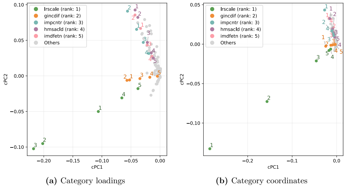
Fig. 24: Category loadings and coordinates of the top-5 variables along cPC1 (cMCA Con vs Lab, ESS 2018)
