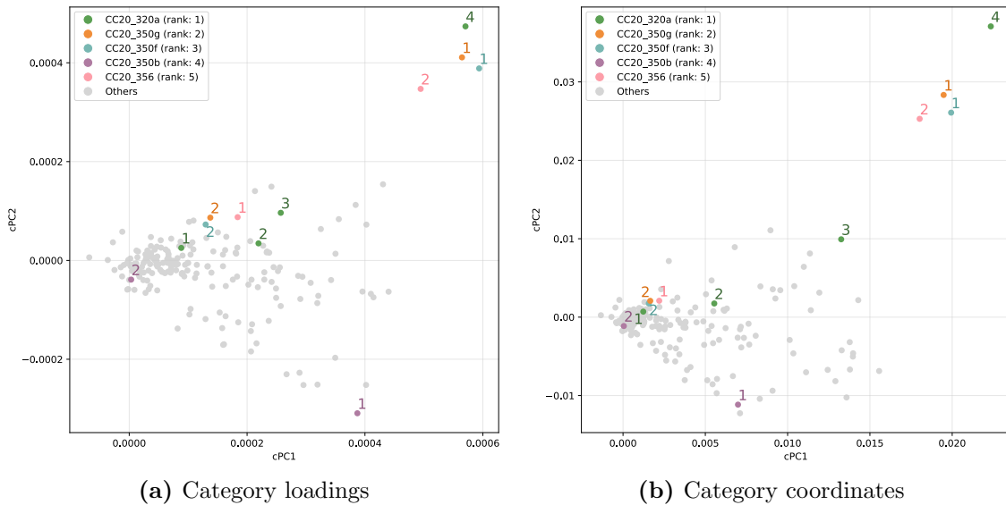
Fig. 21: Category loadings and coordinates of the top-5 variables along cPC2 (cMCA Rep vs Dem, CES 2020)
