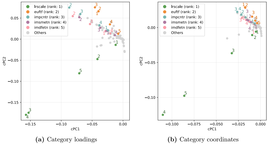
Fig. 23: Category loadings and coordinates of the top-5 variables along cPC2 (cMCA Lab vs Con, ESS 2018)
