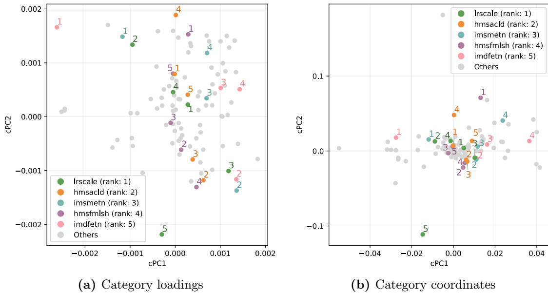
Fig. 27: Category loadings and coordinates of the top-5 variables along cPC2 (cMCA Lab vs UKIP, ESS 2018)
