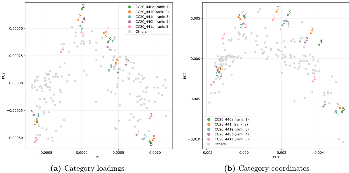
Fig. 16: Category loadings and coordinates of the top-5 variables in Table 10 (MCA, CES 2020)
